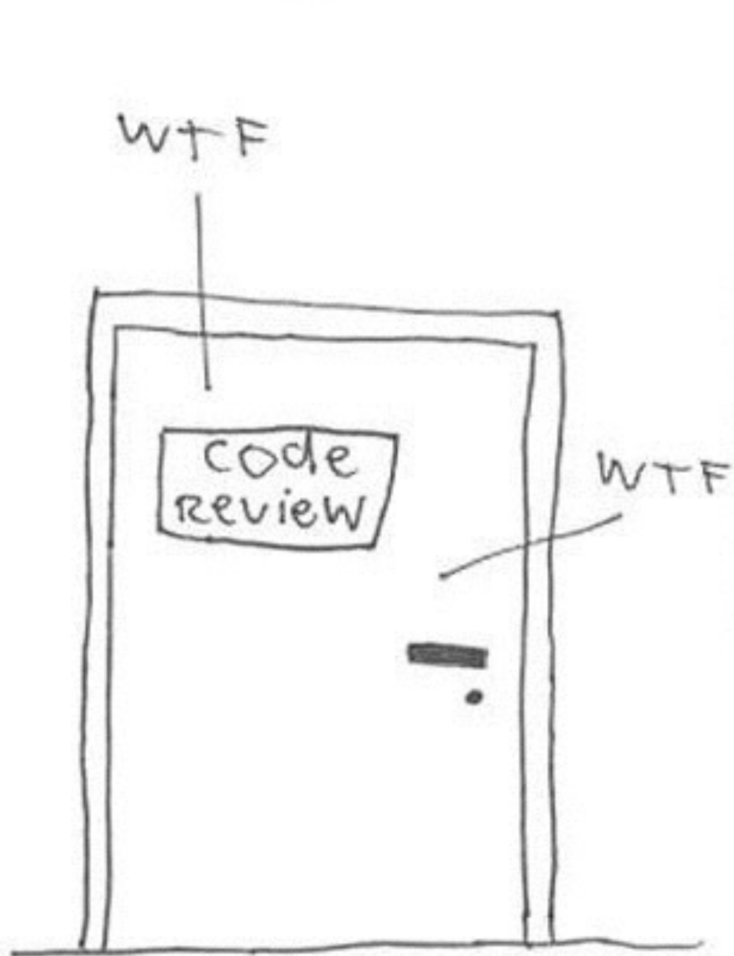
Good code.
